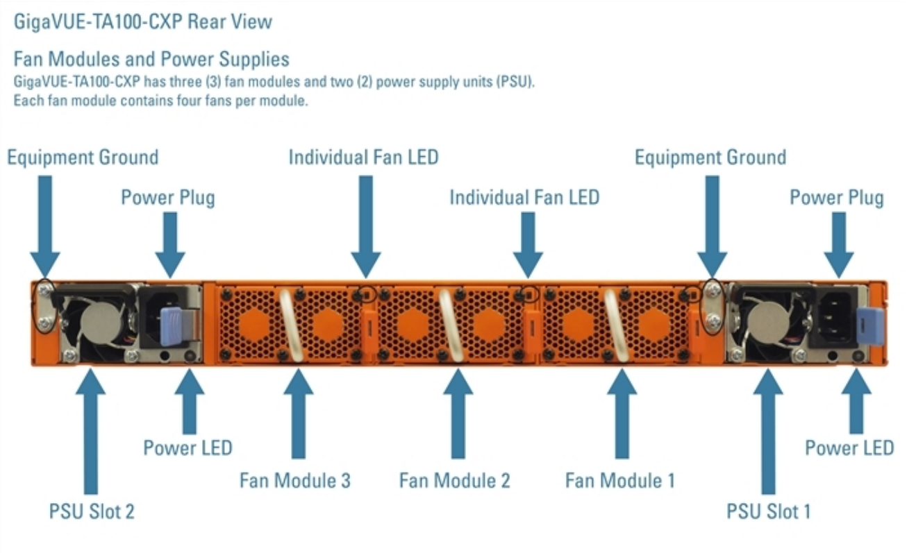
Figure 6 The GigaVUE-TA100-CXP Chassis Rear View
