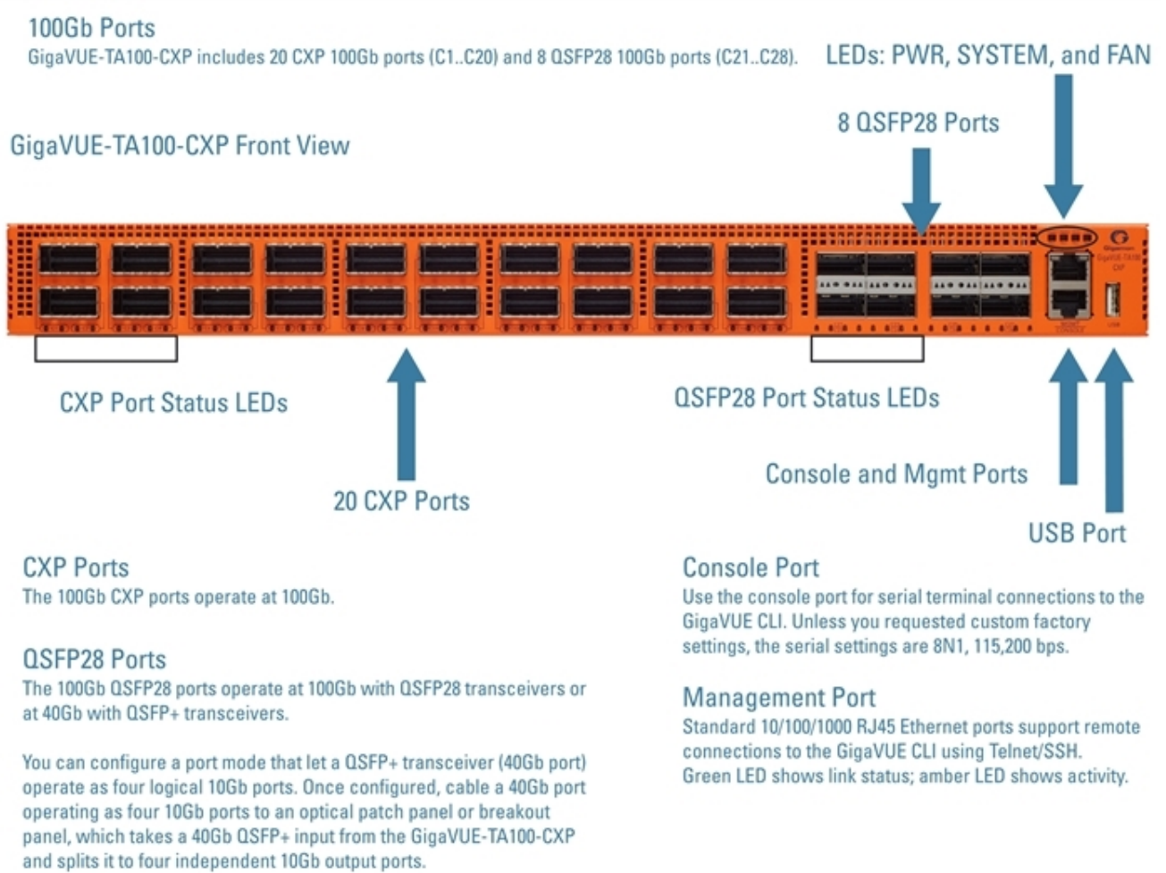
Figure 5 The GigaVUE-TA100-CXP Chassis Front View
