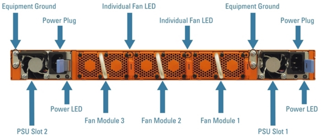
Figure 4 The GigaVUE-TA100 Chassis Rear View
